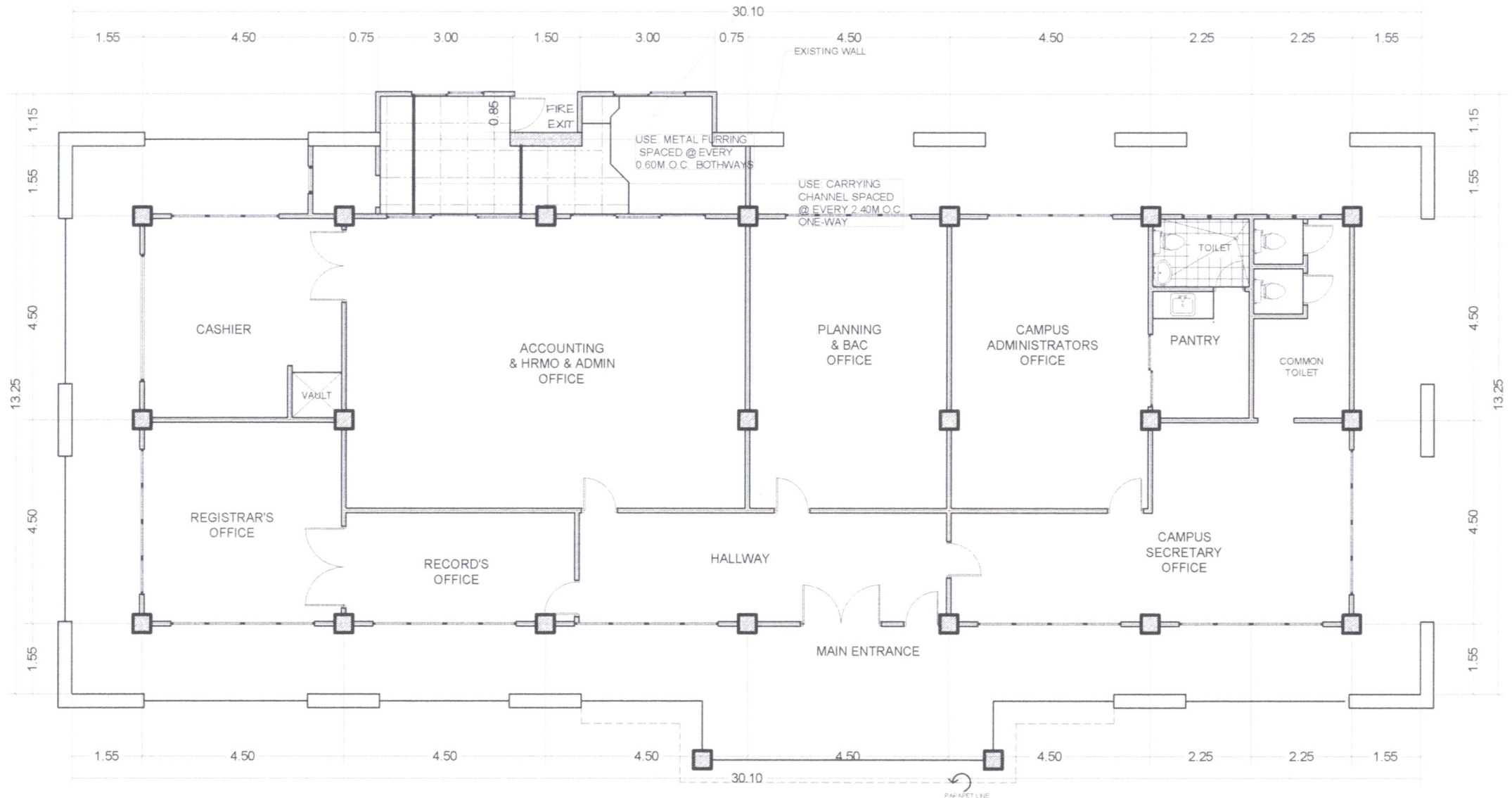
REFLECTED CEILING PLAN SCALE: 1:110MTS
