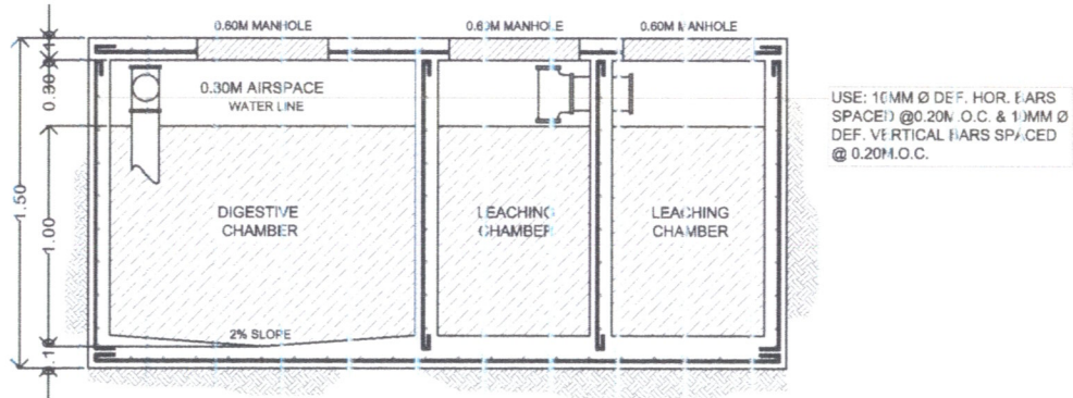
○ SEPTIC VAULT DETAIL SCALE: 1:35MTS
