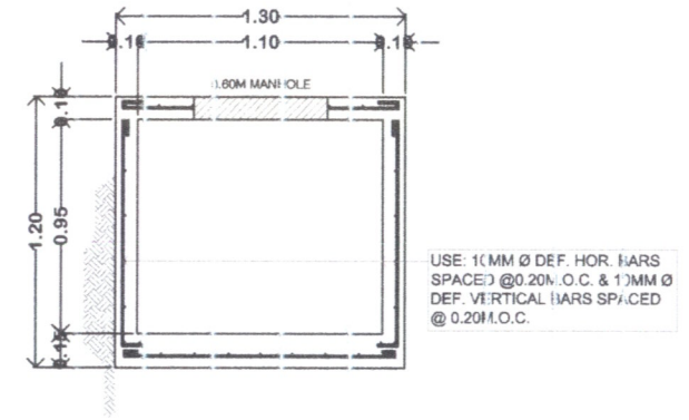
○ CATCH BASIN DETAIL SCALE: 1:35MTS
