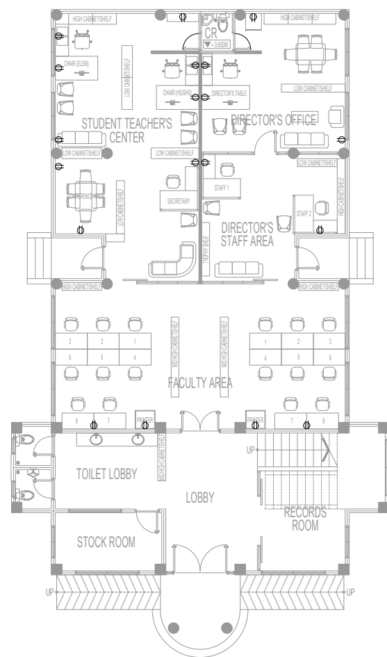
1 GROUND FLOOR ELECTRICAL PLAN A-02 SCALE 1:150 M
