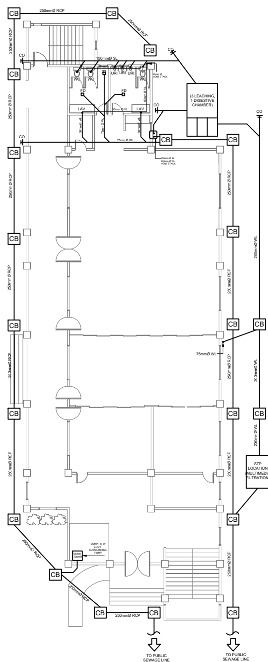
GROUND FLOOR SANITARY PIPING LAYOUT
