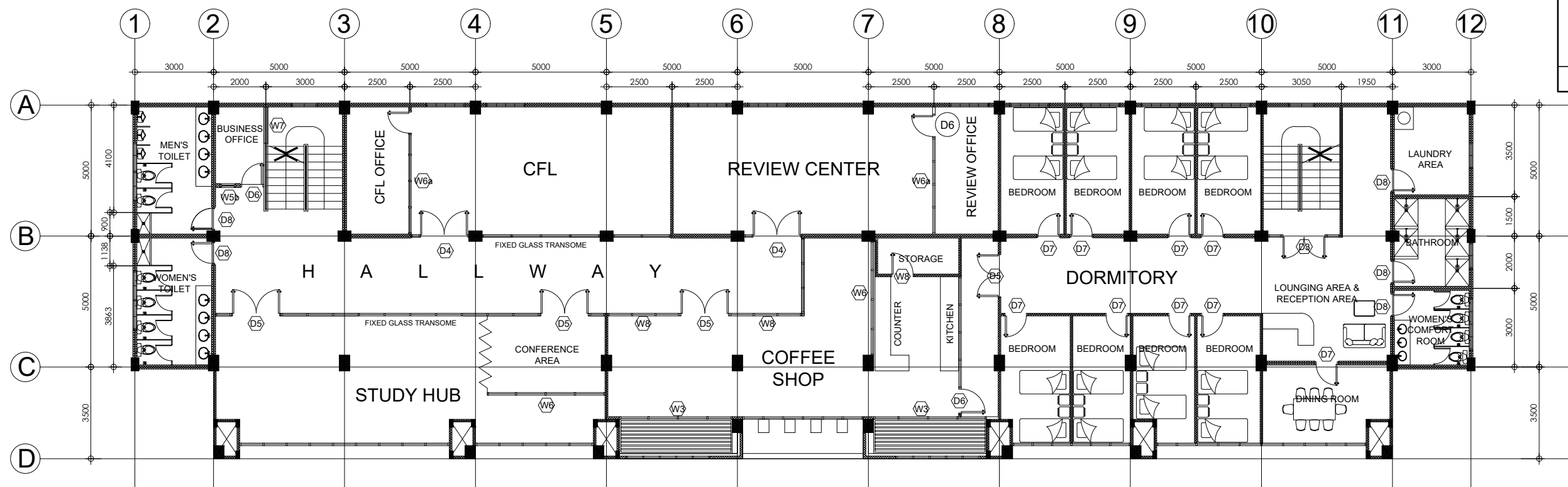
1 SECOND FLOOR PLAN
