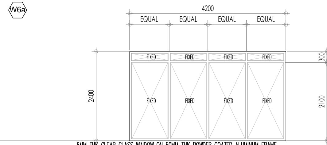
6MM THK CLEAR GLASS WINDOW ON 50MM THK POWDER COATED ALUMINUM FRAME, VERIFY ARCHITECT'S DESIGN FOR APPROVAL, FIXED TYPE
