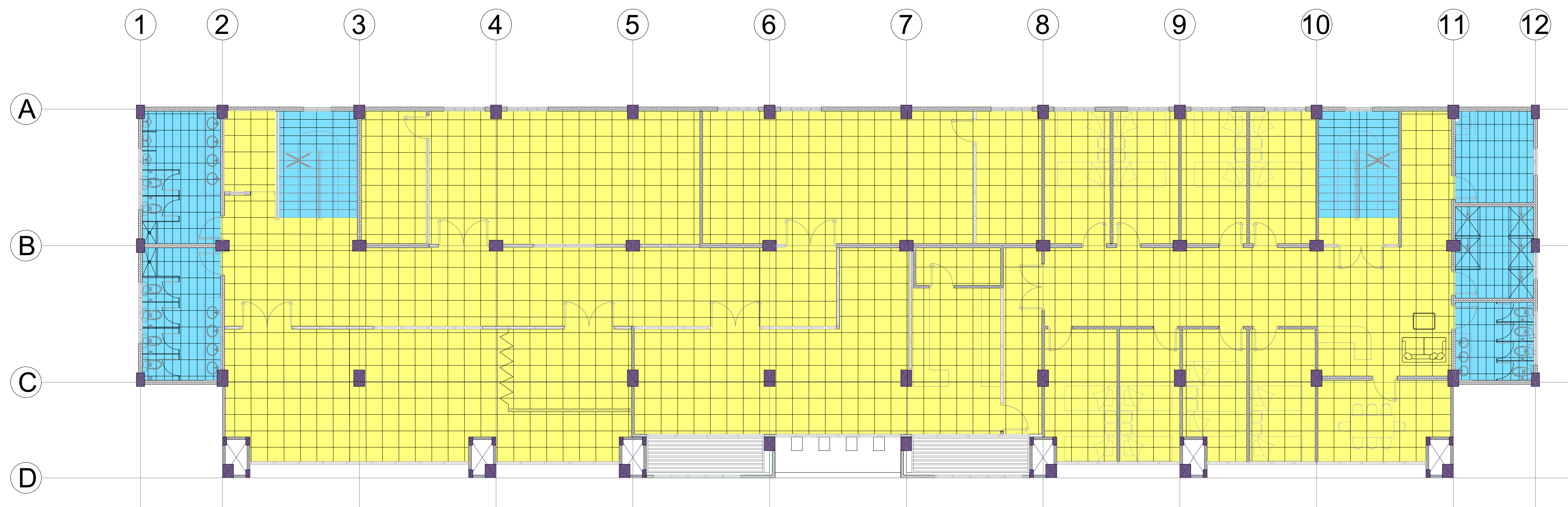
1 SECOND FLOOR TILE LAYOUT
