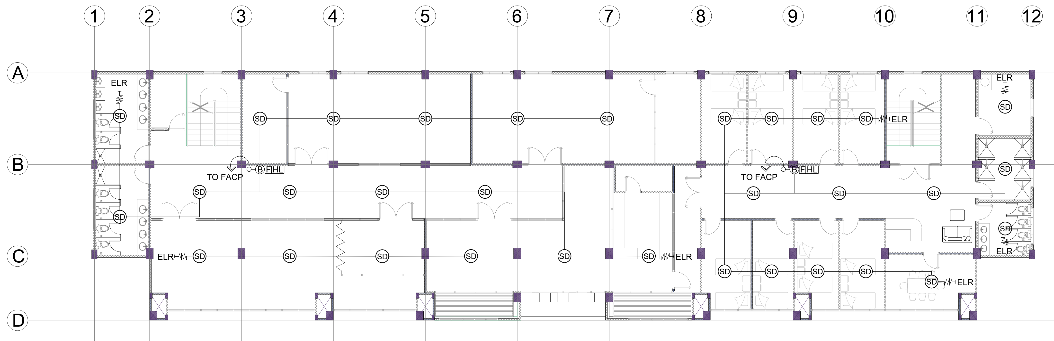
1 2ND FLOOR FIRE DETECTION AND ALARM SYSTEM (FDAS) LAYOUT
