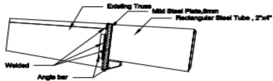
○ Details 1 Halfway Truss Connection to Existing Beam
