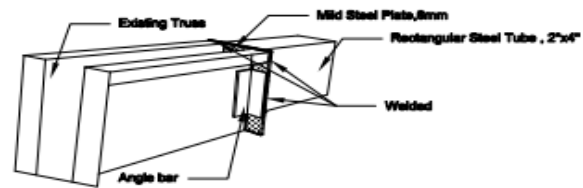
○ Details 2 Halfway Truss Connection to Existing Beam
