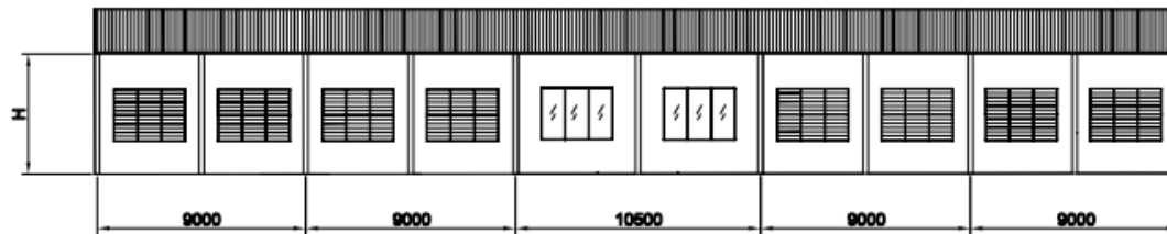
○ Rear Elevation
