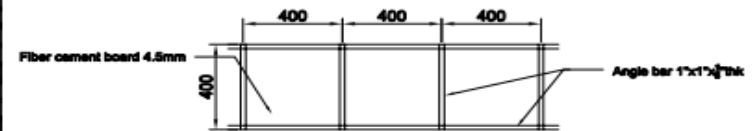
○ Fascia Details
