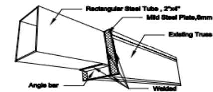
○ Details 2 Halfway Truss Connection to Existing Beam
