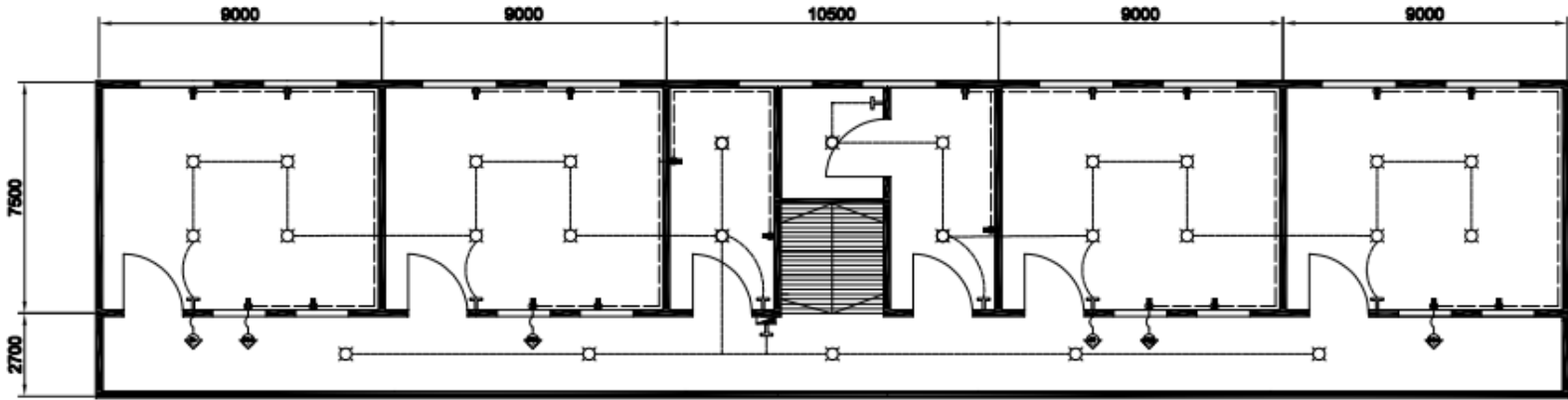
○ LIGHTING AND POWER LAYOUT
