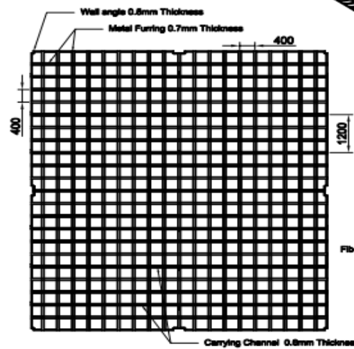
○ Ceiling Support Details
