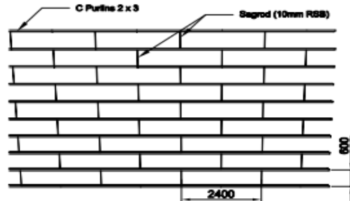
○ Roof Support Details
