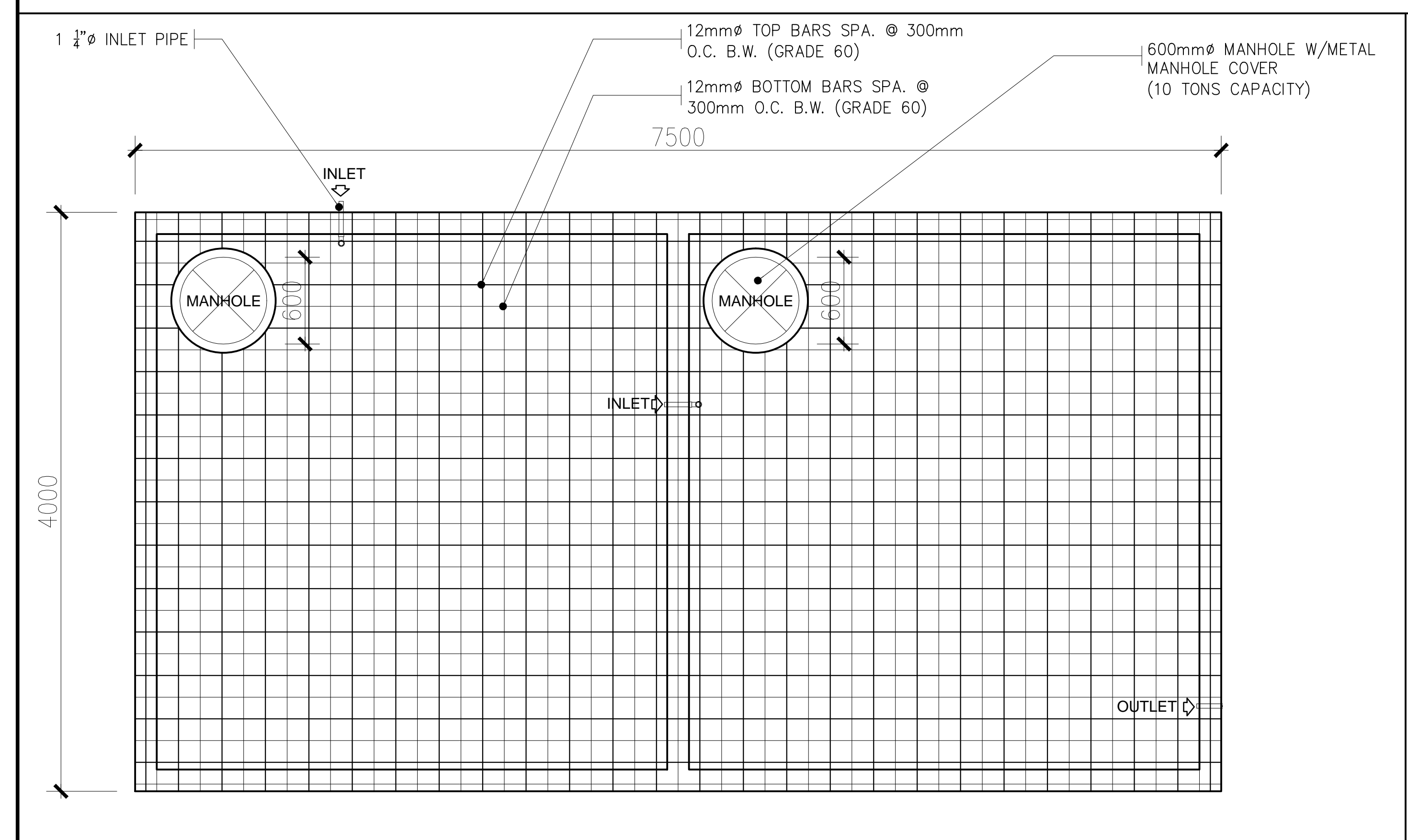
PROPOSED PLAN SCALE 1:25M
