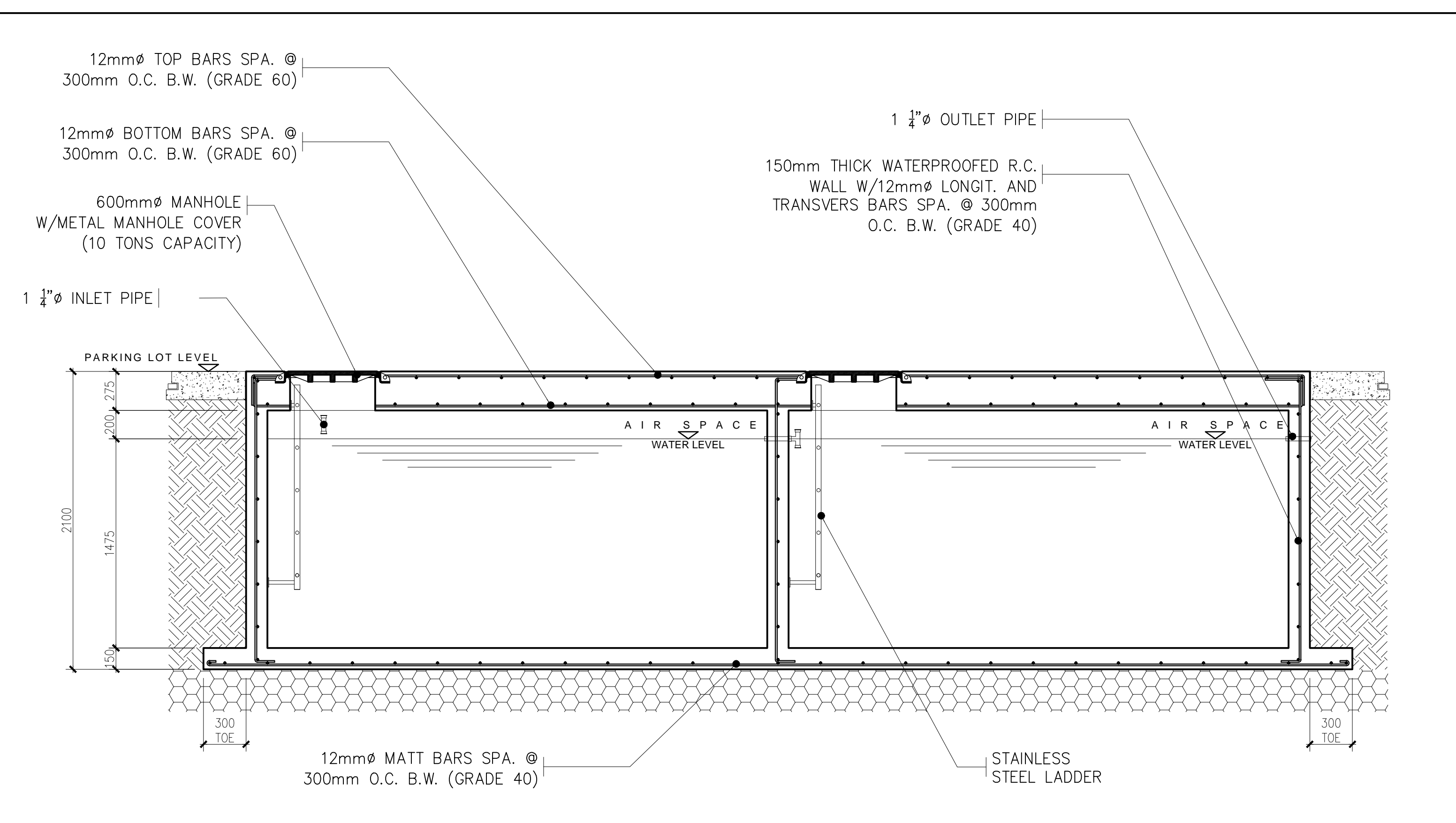
SECTION DETAIL SCALE 1:25M
